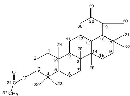
Figure 2. Structure of compound 2 (acetyl lupeol)
