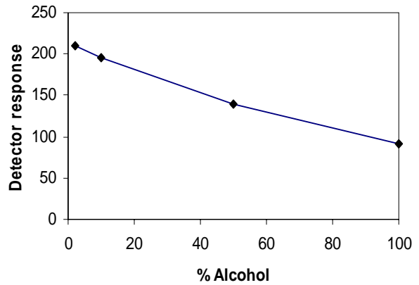
Figure 4. Influence of percent of ethanol on sensitivity of detector.
