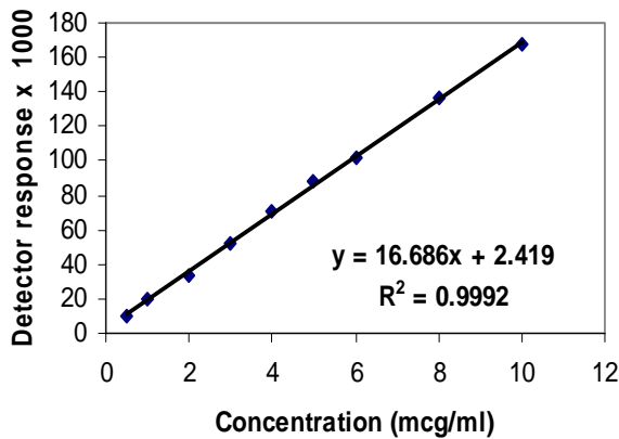
Figure 3. Calibration curve for fentanyl solution.
