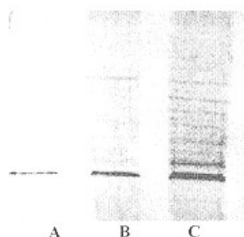
Fig. 2 Sodium dodecyl sulfate polyacrylamide gel electrophoresis of crude dextranases. Samples containing equal volume of each enzyme solution (40-80 \mu g prot/ml), were loaded into each well. (A) Leuconostoc mesenteroides PTCC 1059; (B) 1059M5; (C) 1059M5E4.
