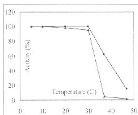
Fig. 3 Temperature stability of dextranases of ▲, Leuconostoc mesenteroides PTCC 1059; ■, mutant 1059M5E4.
