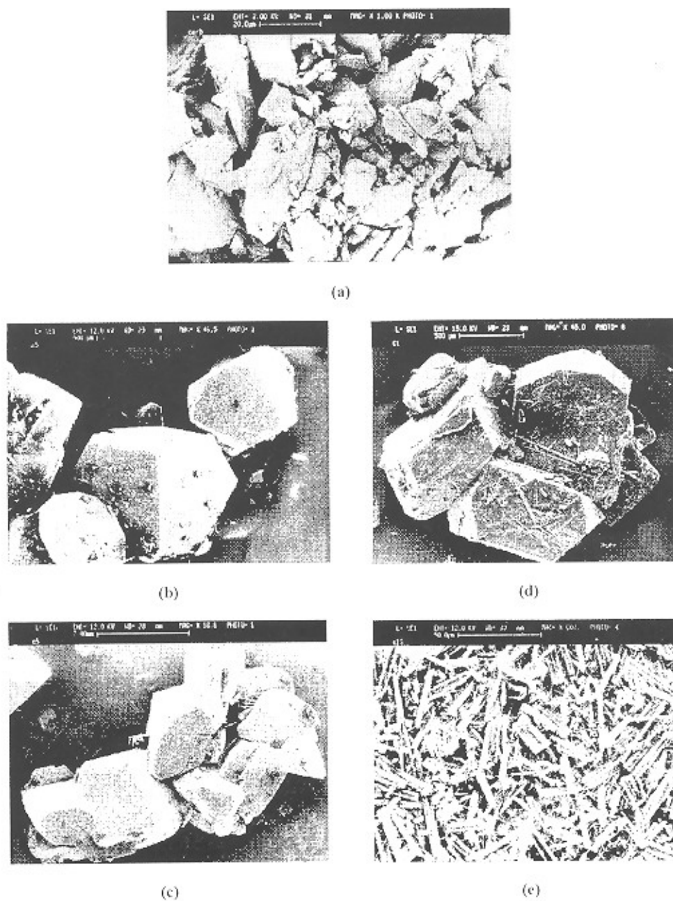
Figure 1. Scanning electron micrographs of (a) untreated carbamazepine, (b) carbamazepine crystallized from alcohol by method 1, (c) method 2, (d) method 3 and (e) method 4.
